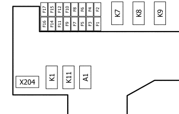
E-Kasten vom Motorraum E-box from engine bay
